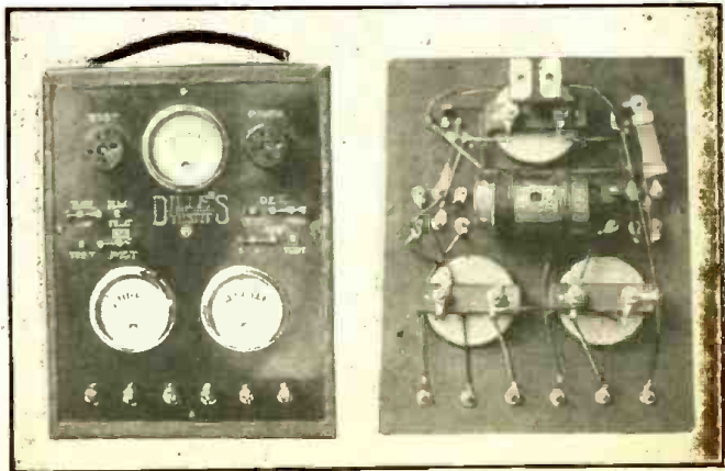
Mr. Alf. E. Dille, of Grinnell, Iowa, built this tube and set tester away back when the "X" base first came out and when most of the radio tubes were of the 200 and 201A types. This was even before the "C" batteries came into general use. Notice the old-fashion sockets, knife switches, and magnetic-vane type meters used on the front panel.
