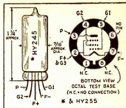
Fig. 3. Tube dimensions and connections. In this illustration, the new tiny pentode is shown in its actual size. Its connections are indicated with reference to an octal base. The types HY245 and '255 hearing-aid tubes are identical in appearance and terminal connections.
