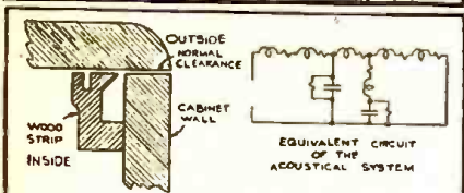
Tone Guard and Equivalent Circuit
