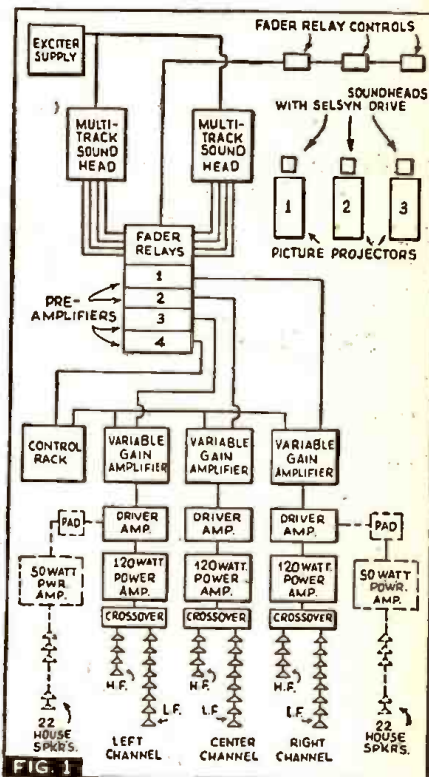
Fig. 1. Simplified block diagram of the "Fantasound" reproducing system. It should be kept in mind that in the Broadway Theatre installation in New York the house speakers indicated (dotted) on the right and left sides of the diagram are not installed in quite this manner although they were part of the system when it was installed in the Disney Studios in Hollywood. In New York, the arrangement is: orchestra, 16 low-level cone loudspeakers at rear, and 3 more on either side; balcony, 2 medium-power hi-fi cone and honeycomb-horn combinations at rear and 2 more on either side, and 16 low-level cone speakers on either side. Thus every seat is literally "bathed" in non-directional or directional sound, as desired, by using these house speakers and the 3 on-stage channels.
