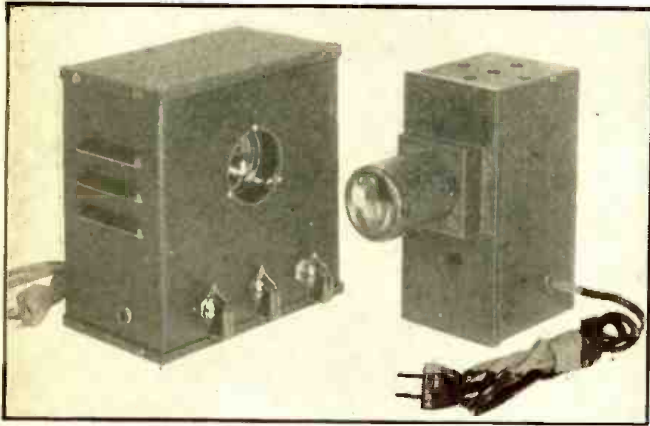
A commercial type of photocell equipment suitable for use in electronic burglar alarm systems. Left, photocell equipment in its housing; right, the exciter (light source). Photos—Worner Products Co.
