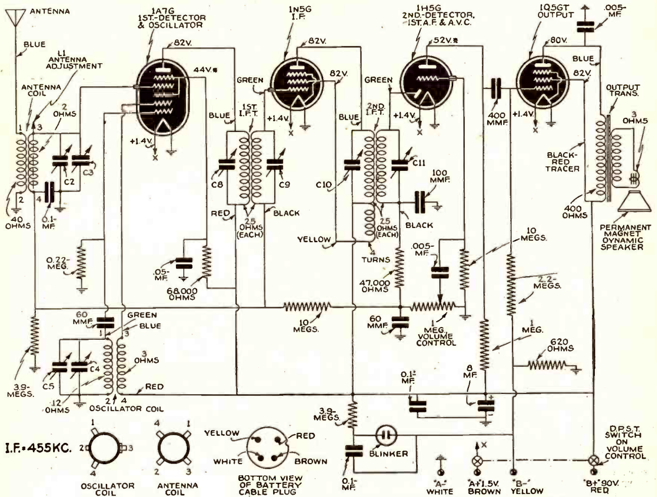
Complete schematic diagram of the RCA Victor Model BT-42, Battery-operated Superhet., Chassis No. RC-408A.
