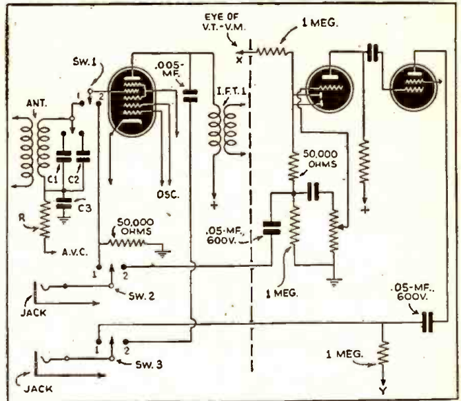
Diagram of "Signal Substituter". The switches operate as follows: Sw. I: pos. 1, receives signal tuned by trimmer; pos. 2, receives untuned signal fed in by probe. Sw. II: pos. 1, connects probe to grid of converter (through Sw. I, pos. 2); pos. 2, ditto, of 1st A.F. for Audio In. Sw. III: pos. 1, connects probe 2 to plate of output for Audio Out; pos. 2, ditto, of converter for R.F. Out.
